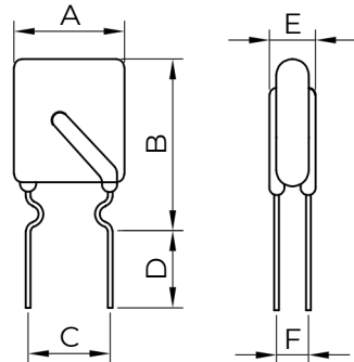
RLD30P090U~RLD30P250U LEAD DIA: Ø0.51mm LEAD SIZE: 24AWG
