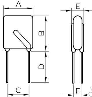
RLD30P300U~RLD30P900U LEAD DIA: Ø0.81mm LEAD SIZE: 20AWG
