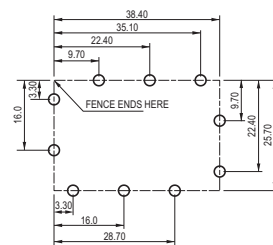
EXAMPLE:- MOUNTING HOLE PATTERN FOR 10 & 20 SERIES
