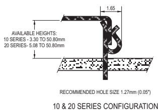
10 & 20 SERIES CONFIGURATION
