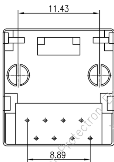
BOTTOM VIEW
