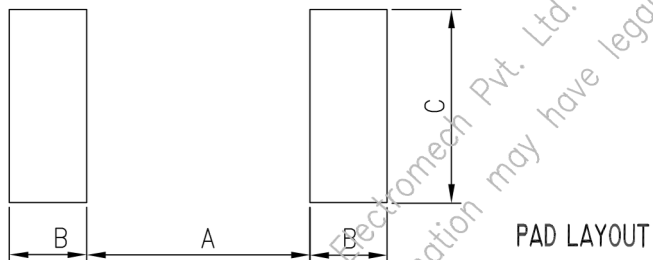
Pad Dimensions (Millimeters)
