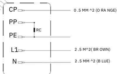
CABLE CONNECTION DETAILS
