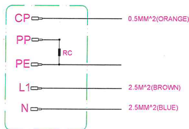
CABLE CONNECTION DETAILS
