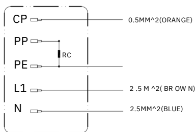
CABLE CONNECTION DETAILS
