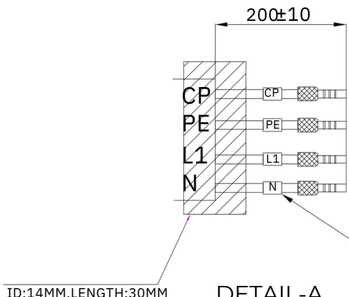
DETAIL-A CABLE SIZE DETAILS
