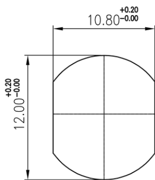
MOUNTING DETAILS
