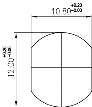
MOUNTING DETAILS
