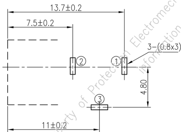
PCB LAYOUT
