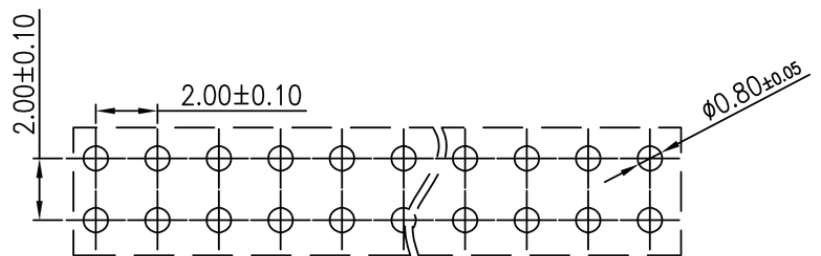
RECOMMENDED P. C. BOARD LAYOUT
