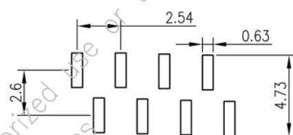
RECOMMENDED PCB LAYOUT (SURFACE MOUNT B1 TYPE)
