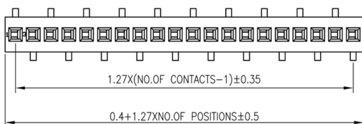
SURFACE MOUNT B1 TYPE
