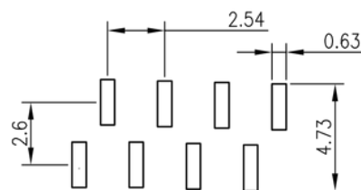
RECOMMENDED PCB LAYOUT (SURFACE MOUNT B2 TYPE)
