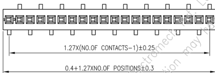
SURFACE MOUNT B2 TYPE
