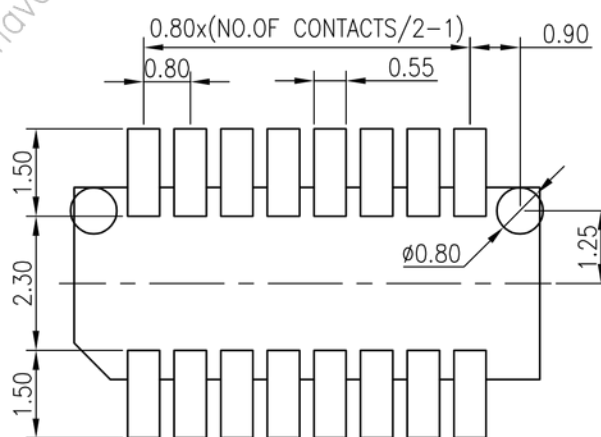
RECOMMNEED P.C.BOARD LAYOUT
