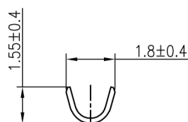
SEC-BB
