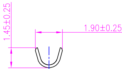
SEC-BB
