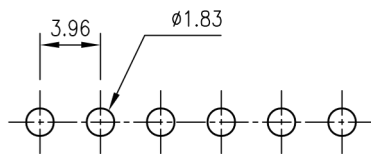
PCB HOLE DIMENSIONS
