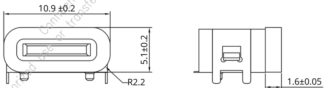
GASKET DETAILS
