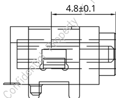
MATING PART INSERTION
