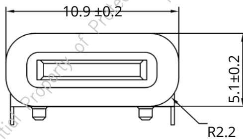
GASKET DETAILS
