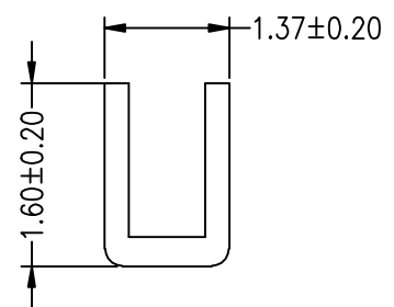
SEC: C-C
