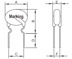
RLD120P010X ~ RLD120P090X Lead Size : 22AWG Ø 0.65mm
