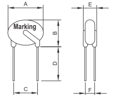
RLD120P110X ~ RLD120P375X. Lead Size : 20AWG Ø 0.81mm
