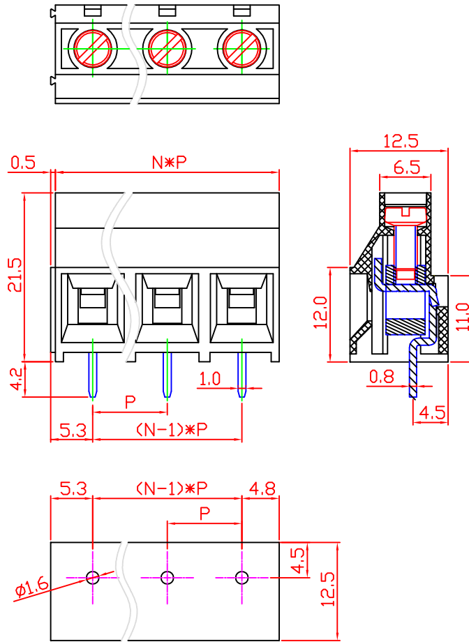
PCB LAYOUT
