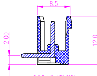
P.C.B MOUNTING(R)
