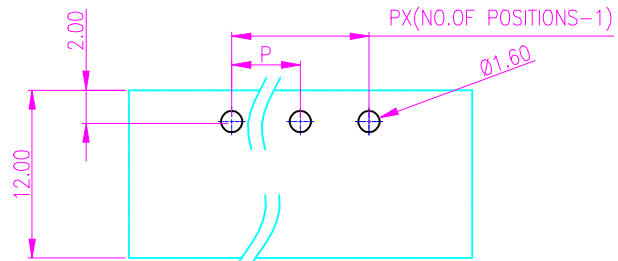
RECOMMENDED PCB LAYOUT(R)
