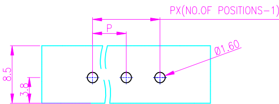
RECOMMENDED PCB LAYOUT(V)
