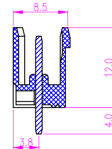
P.C.B MOUNTING(V)
