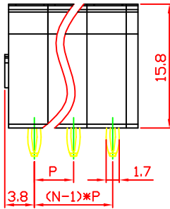
Contact type(P)
