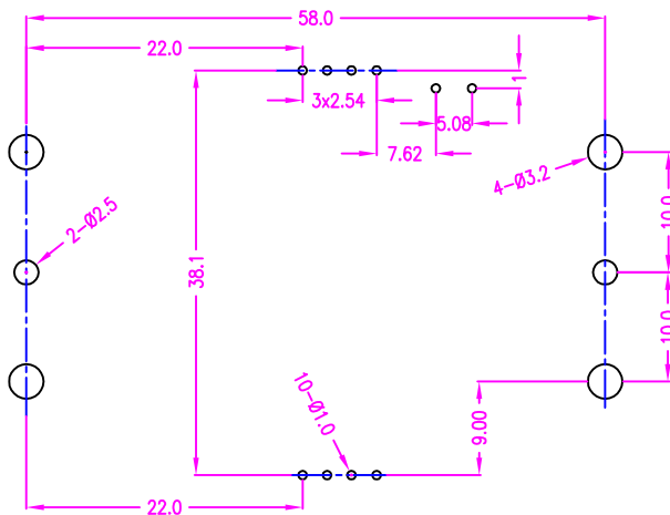
MOUNT LAYOUT
