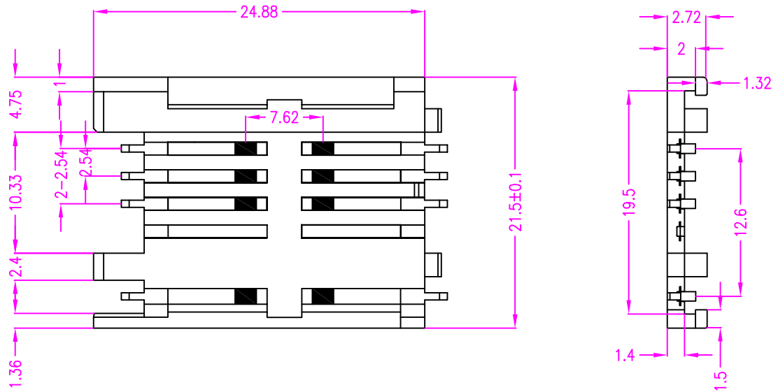
INTERNAL CONSTRUCTION W/O DRAWER
