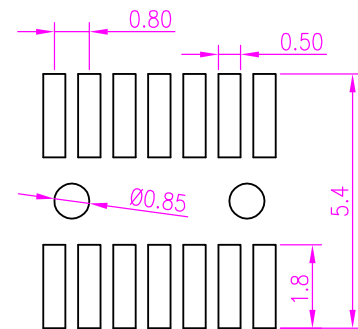
RECOMMENDED PCB LAYOUT(TOP SIDE) (PCB TOLERANCE ±0.05)
