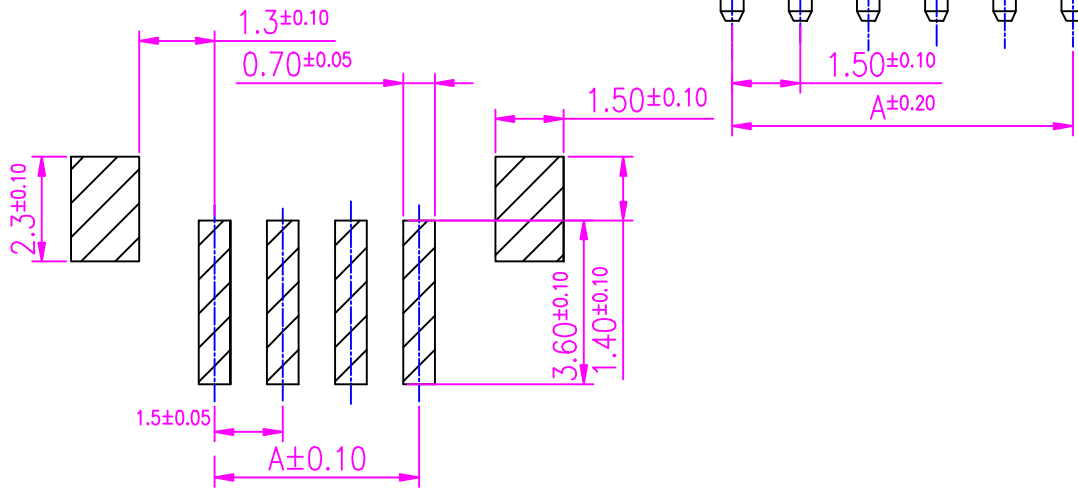
PCB LAYOUT
